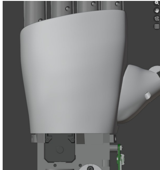
Figure 5.75: Skeleton - Upper cover installed
