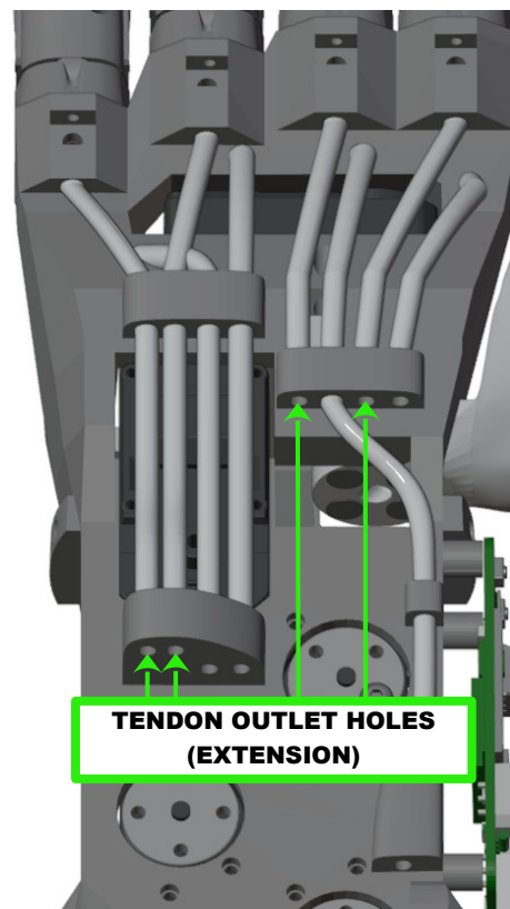
Figure 5.48: Tendon outlet holes (extension)
