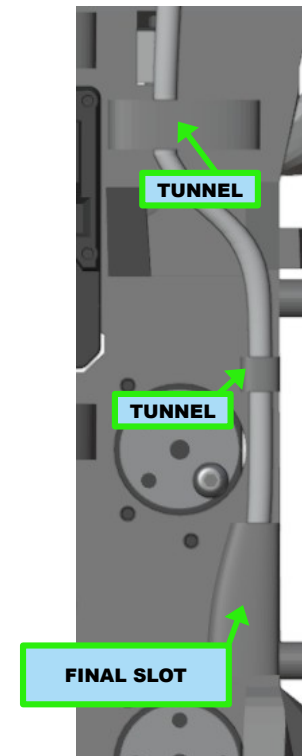
Figure 5.29 : Inserting the tube into the two pass-through tunnels and then into the final slot (rear view)
