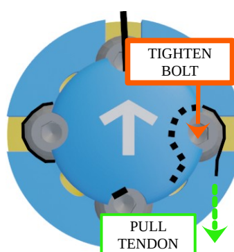
Figure 5.65: Flexion end: pulling and securing
