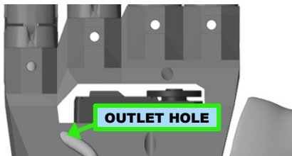
Figure 5.40 : Inserting the tube into the tendon outlet hole (rear view)
