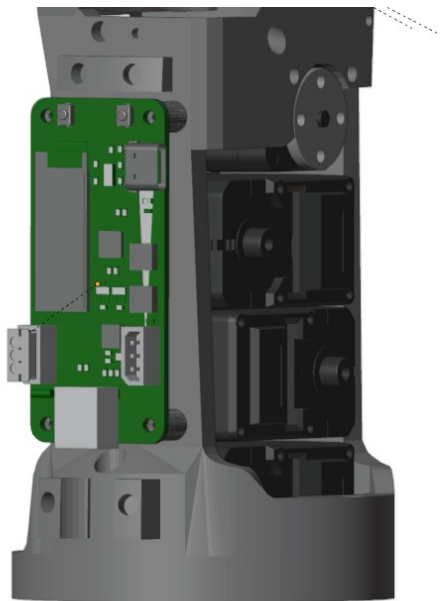
Figure 5.15: Logic board installed
