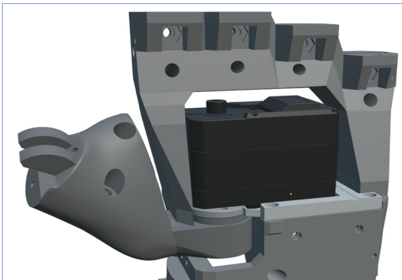
Figure 5.6: TRS and TRS Platform installed on the skeleton
