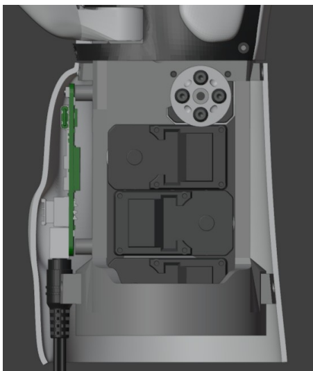
Figure 5.79: Skeleton - Front lower cover area
