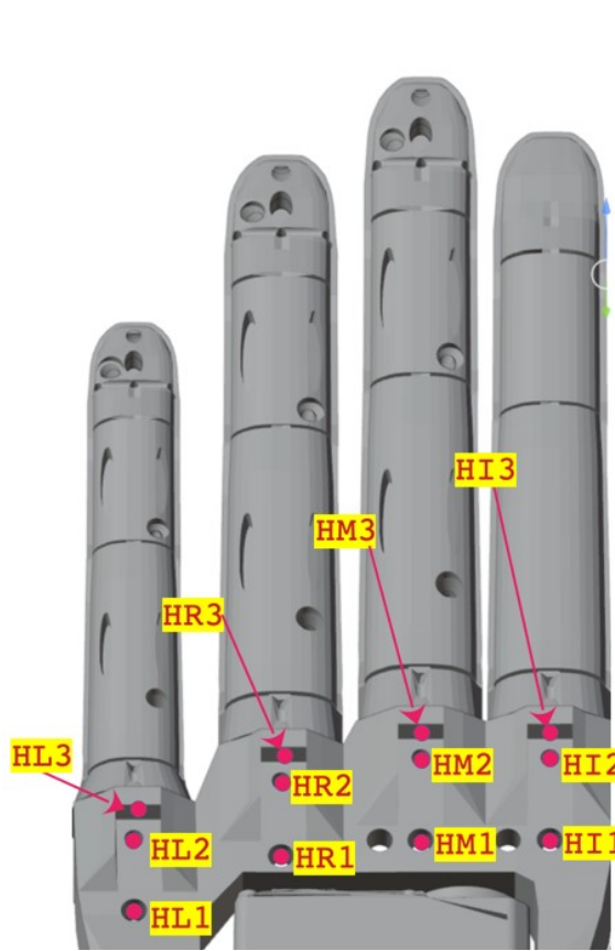
Figure 14.8: Left hand - rear view - tendon holes
